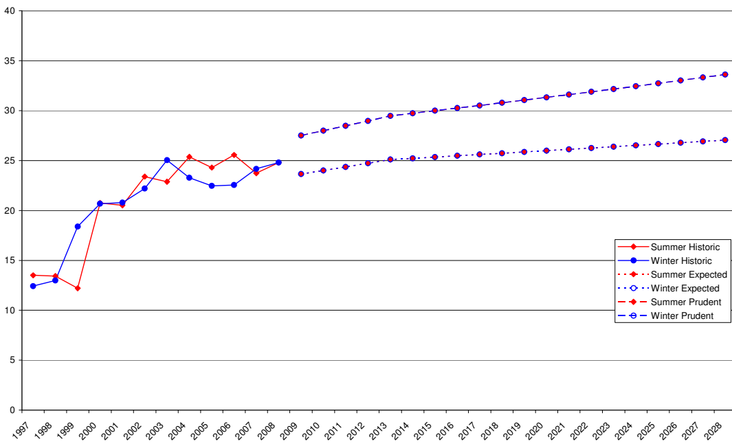
Figure 29: Naseby GXP Load Forecast
