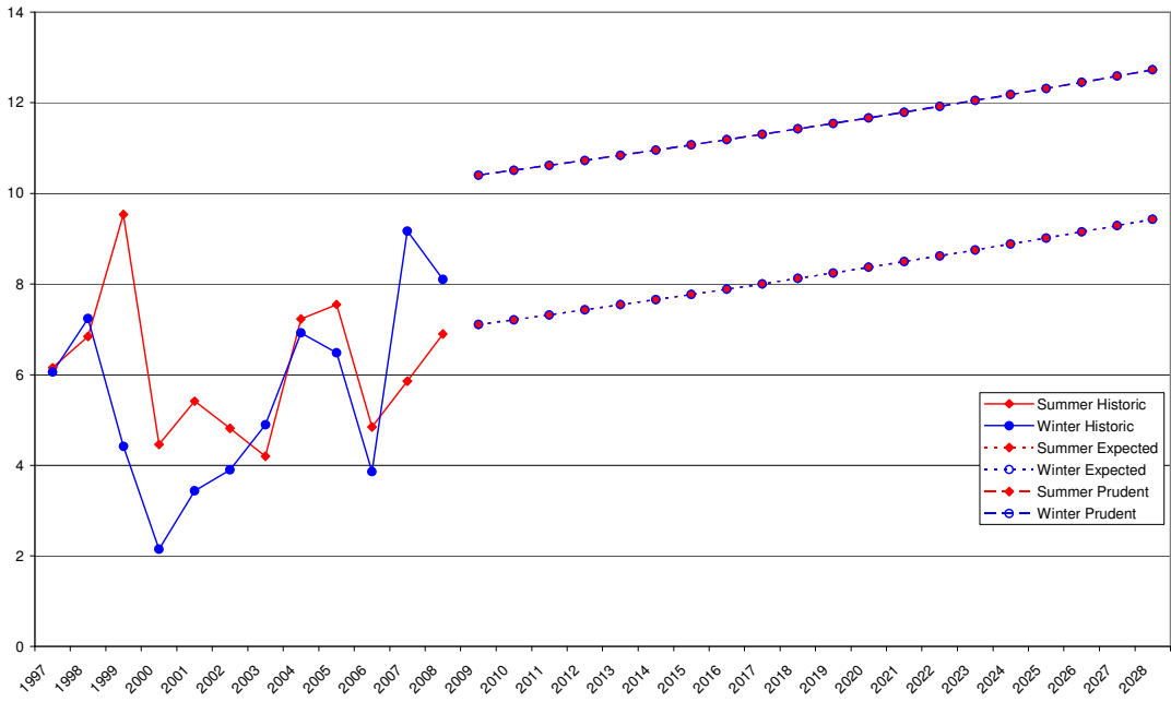
Figure 22: Clyde GXP Load Forecast
